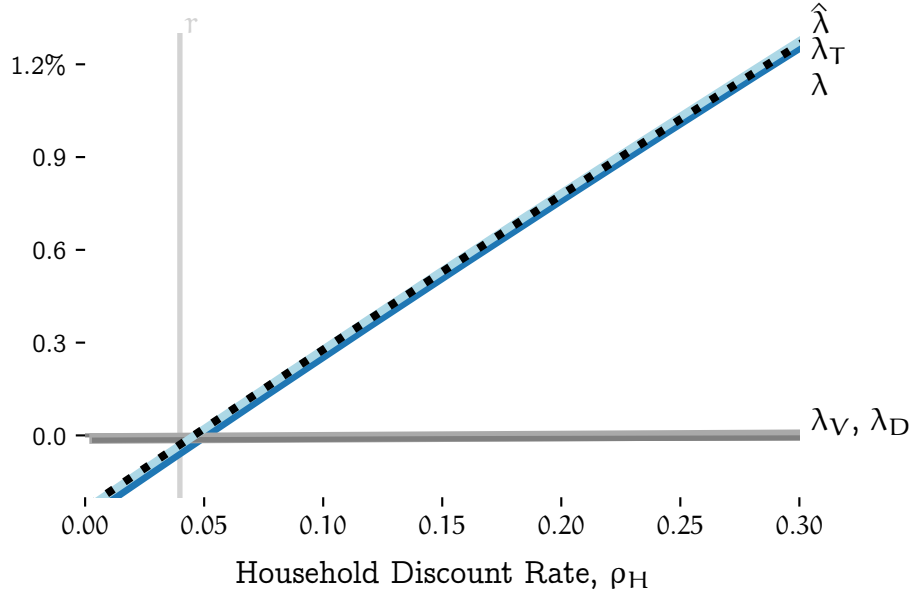
Figure 4: The x-axis is the annualized household discount rate. The y-axis represents the welfare gains in percentage points of consumption. The vertical line corresponds to the (annualized) international interest rate.
