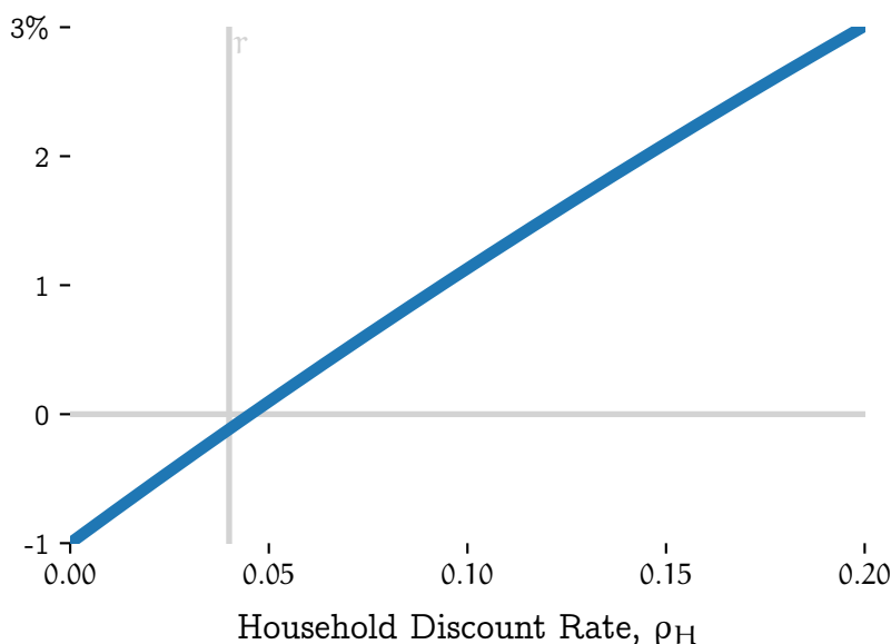
Figure 2: The solid thick line represents the value of \hat{\lambda} (y-axis) as a function of the household discount rates \rho_H (x-axis) assuming \rho_G = 0.20 . The vertical line represents the market discount rate, r = 0.04 . The horizontal solid line represents \lambda = 0 .
