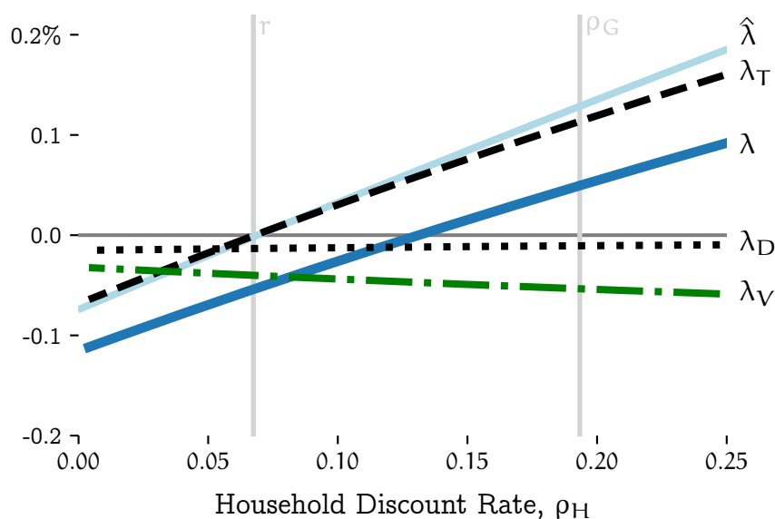
Figure 6: The x-axis is the annualized household discount rate. The y-axis represents the welfare gains in percentage points of consumption. The two vertical lines corresponds to the (annualized) international interest rate and the government discount rate.
