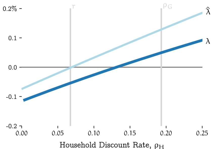
Figure 5: The x-axis is the annualized household discount rate. The y-axis represents the welfare gains in percentage points of consumption. The two vertical lines corresponds to the (annualized) international interest rate and the government discount rate.
