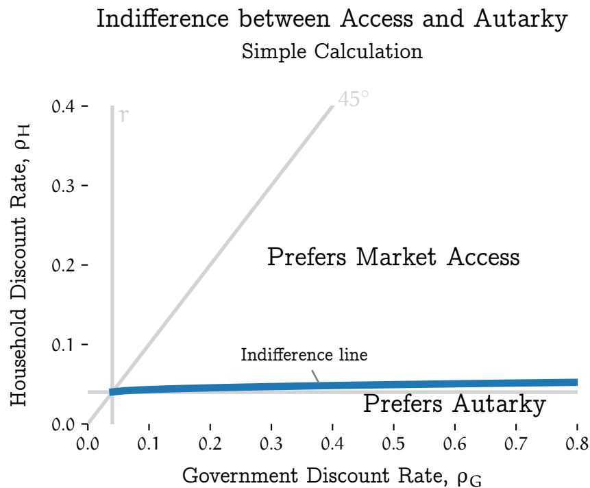
Figure 1: Values of \rho_H above the solid thick line represent values for which the households strictly prefer access to financial markets over autarky. Values below are those where the opposite is preferred. The indifference points are captured by the solid thick line. The vertical and horizontal lines represent the market discount rate.
