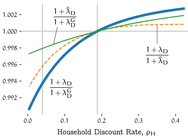
Figure 11: The two vertical lines represent the market interest rate and the discount factor of the government in the CE calibration.
