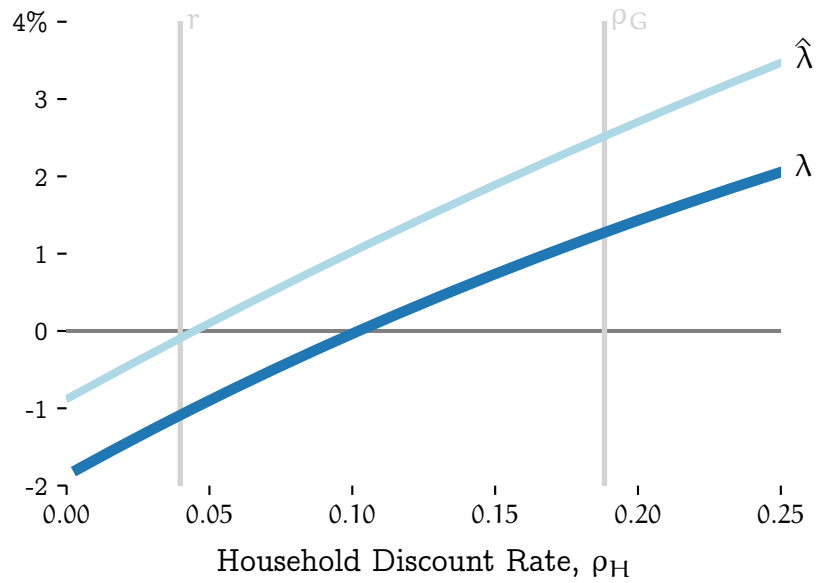
Figure 7: The x-axis is the annualized household discount rate. The y-axis represents the welfare gains in percentage points of consumption. The two vertical lines corresponds to the (annualized) international interest rate and the government discount rate.
