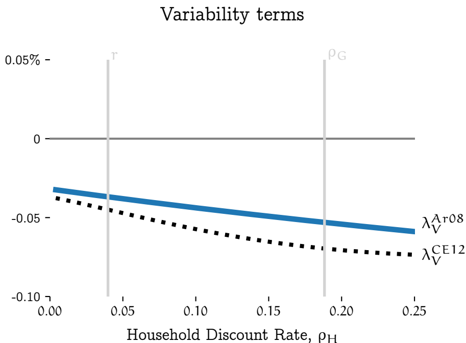
Figure 8: The x-axis is the annualized household discount rate. The y-axis represents the welfare gains in percentage points of consumption. The two vertical lines corresponds to the (annualized) international interest rate and the government discount rate.
