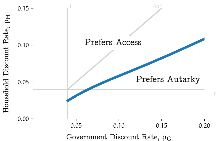
Figure 10: The solid line represents the (annualized) household discount rate (y-axis) that keeps a household indifferent between market access or not, for different (annualized) government discount rates (x-axis). The rest of the parameters are as in the CE calibration.
