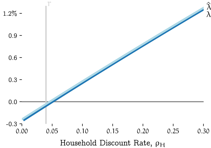
Figure 3: The x-axis is the annualized household discount rate. The y-axis represents the welfare gains in percentage points of consumption. The solid dark line is the results from the Aguiar and Gopinath (2006) calibration. The solid light line is the result from using formula (3). The vertical line corresponds to the (annualized) international interest rate.
