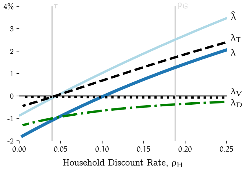
Figure 9: The x-axis is the annualized household discount rate. The y-axis represents the welfare gains in percentage points of consumption. The two vertical lines corresponds to the (annualized) international interest rate and the government discount rate.
